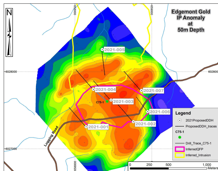
Drilling Locations 2021
